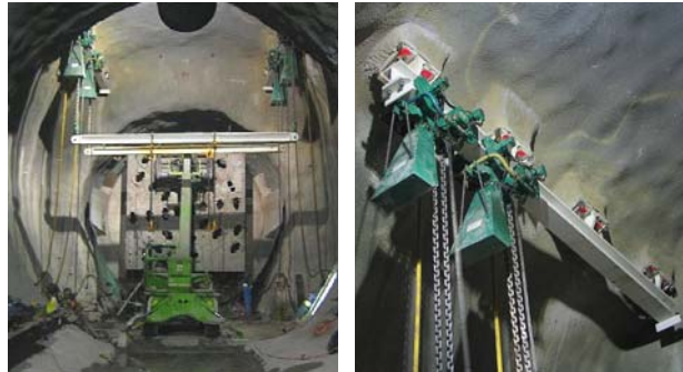
Alp Transit Tunnel: Disassembling works on a tunnel drilling machine with 4 JDN Mono-rail Air Hoists EH 25.
